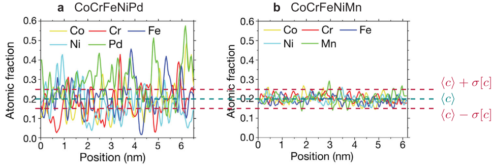
Figure 1. Solute concentrations versus position along [\bar{1}12] in one (\bar{1}\bar{1}1) atom plane, obtained from EDS line scans, in two HEAs (a) CoCrFeNiPd and (b) CoCrFeNiMn. The specimen thickness along [110] is \sim 15 nm, leading to N \approx 60 atoms in each atom column. In a random alloy, the solute concentration in any finite domain of N atoms fluctuates around the mean value \langle c \rangle = \bar{c} with a standard deviation \sigma[c] = \sqrt{\bar{c}(1 - \bar{c})/N} . For \bar{c} = 0.2 and N = 60 , \sigma[c] \approx 0.05 . The measured fluctuations in CoCrFeNiMn are consistent with the random alloy while those in CoCrFeNiPd show significantly larger fluctuations, typically two standard deviations ( \pm 0.10 ) and larger, as indicated in the figure. Note that the average Pd concentration in this particular region of the CoCrFeNiPd alloy actually exceeds the nominal concentration \bar{c} = 0.2 . Figure adapted from Ding et al. [14], reprinted by permission from Springer Nature.
