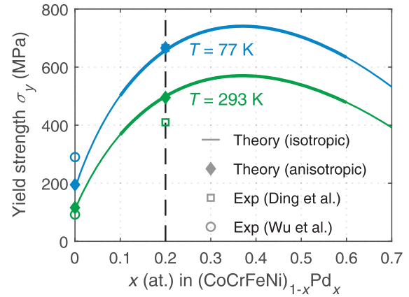
Figure 2. The prediction of initial yield strength of pseudo-binary alloy (\text{CoCrFeNi})_{1-x}\text{Pd}_x as a function of x , at loading strain rate 10^{-3} \text{ s}^{-1} and various temperatures. Here, isotropic theory uses the ROM polycrystal elastic moduli; the anisotropic theory predictions are based on DFT C_{ij} . The experimentally measured yield strengths [14,15] are also indicated. For CoCrFeNi, the strengths shown are from Hall-Petch extrapolation to infinite grain size; for CoCrFeNiPd, the strengths are from experiments at grain size of 135 \mu\text{m} .
